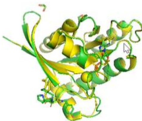
Figure 5: RMSD Calculation 9ggy(green) 9G0Y (yellow)
