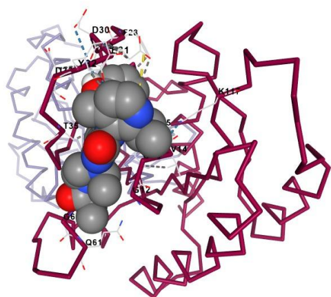
Figure 10: Molecular Docking (Protein-ligand (Sotorasib) interaction score C2(-8.1)
